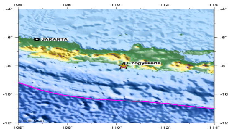
JAVA, INDONESIA 2006 05 26 22:54:01 UTC 8.01S 110.29E Depth: 17.1 km, Magnitude: 6.2 Earthquake Location
